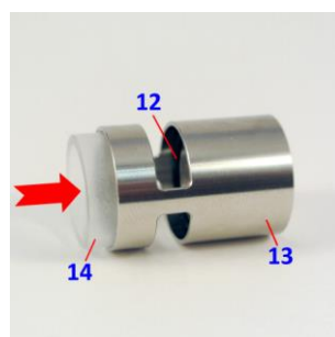
Pic. 19: The glass tank [14] will be inserted into the tank cover [13]. The o-ring [12] seals it.
