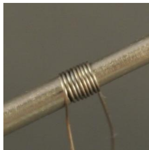
Pic. 2: On a winding aid several turns of resistance wire being formed into a coil.
