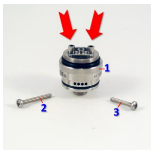
Pic. 5: The long screw [2] is the positive terminal, the short screw [3] the negative. Both are plugged into the base [1] and tightened slightly.
