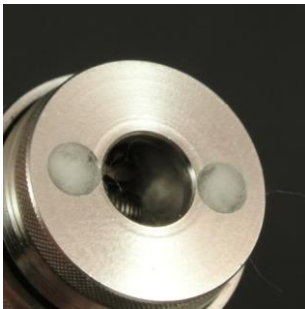
Pic. 5: They should thereby rest on the cotton at the sides of the coil and should be pushed until they no longer protrude from the chamber cap holes.
